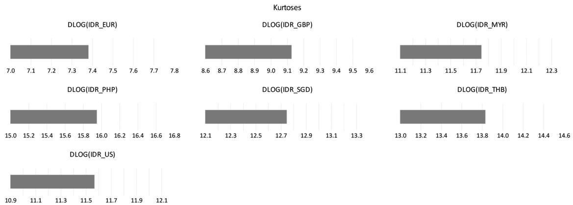
Figure 5. Kurtosis evolution of the 7 exchange rates, in the period from September 3, 2018 to October 20, 2020.
